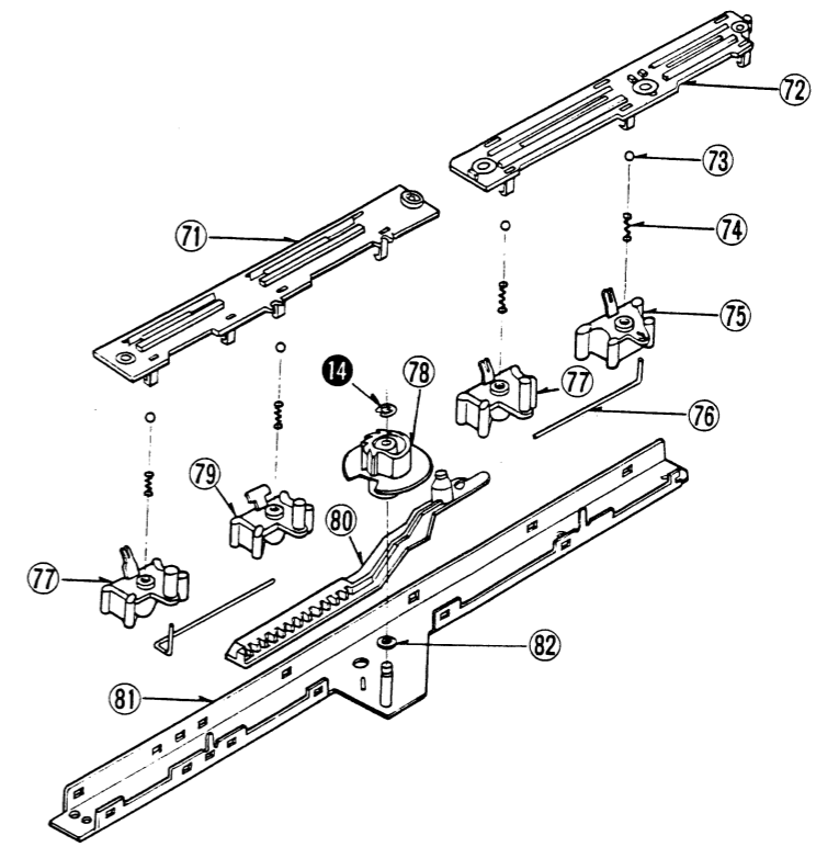
AUTOMATIC MECHANISM ASS'Y
